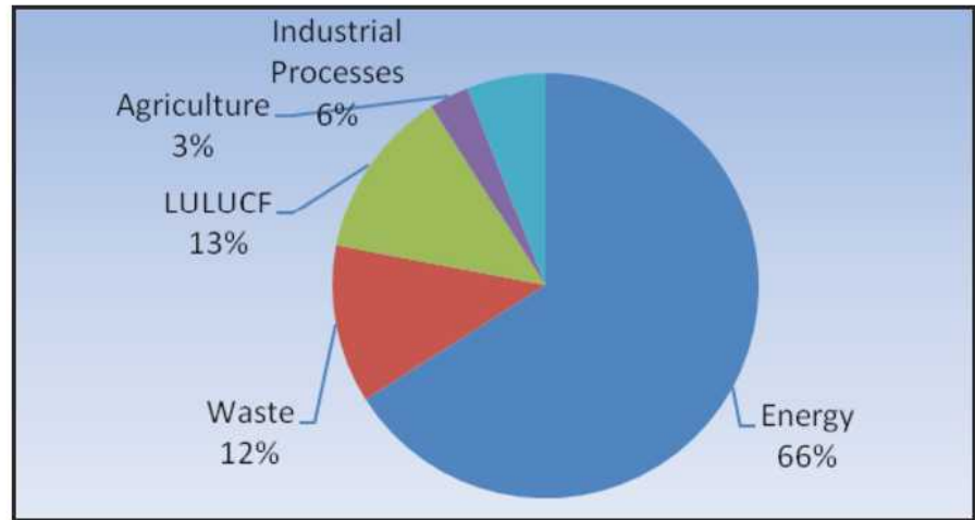
Chart 7.1: Percentage of GHG Emissions by Sector, 2000
