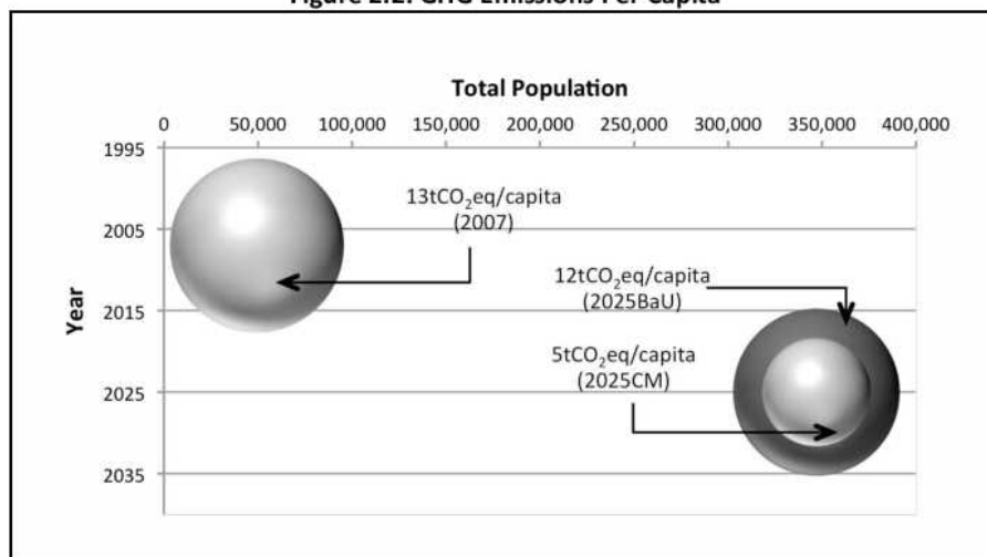
Figure 2.2: GHG Emissions Per Capita
